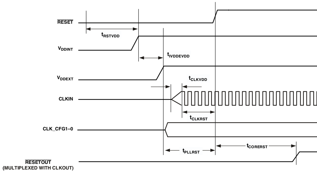
Figure 6. Power-Up Sequencing
